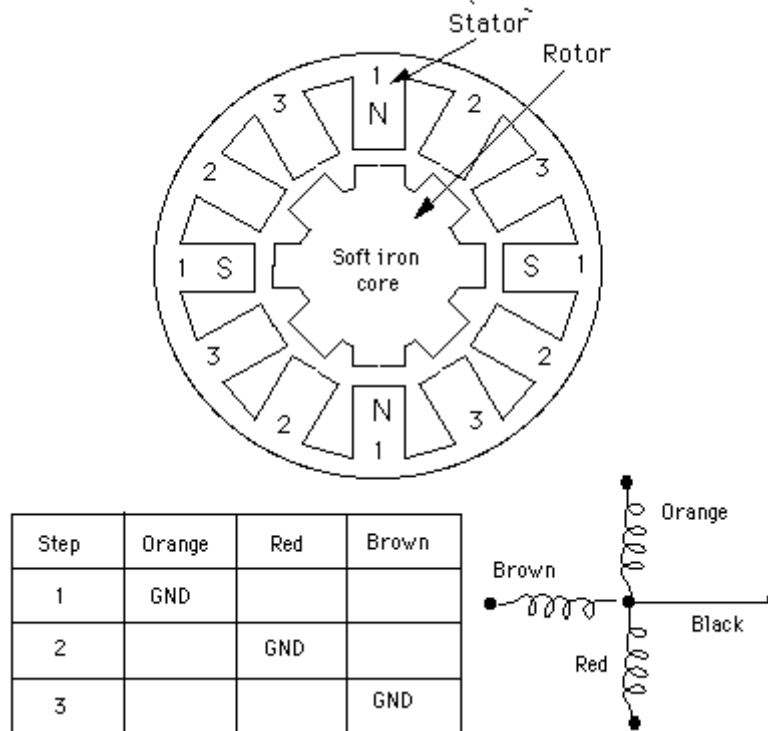
Figure 1. Pole layout for 3-phase stepper motor
